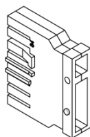
A) Female Cap, Qty. 1
