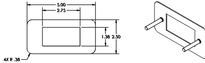
METAL FACEPLATE ONLY (CORDLESS) 1 TELECOM PLATE KNOCKOUT
