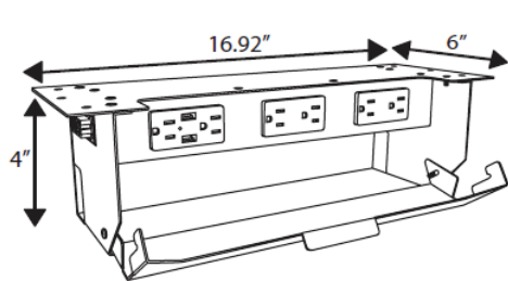
Power Island
