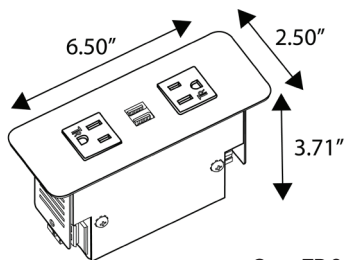
Cove TR 2 Power 2 USB DaisyLink
