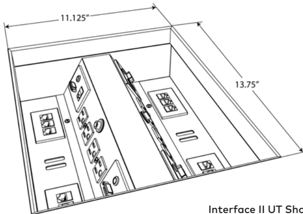
Interface II UT Shown (without Trim Pivot Kit Lid)
