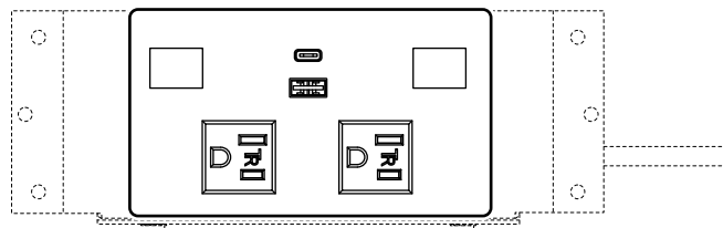
Cutout Opening (5.25in X 3.00in)
