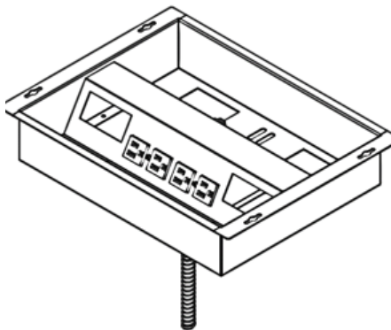
UNDERTABLE HARDWIRED (WITHOUT LID SHOWN)
