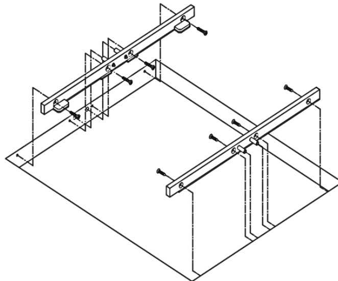
ASSEMBLED TRIM PIVOT KIT COMPONENTS
