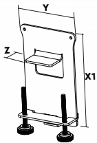
CLAMP-ON BRACKET
