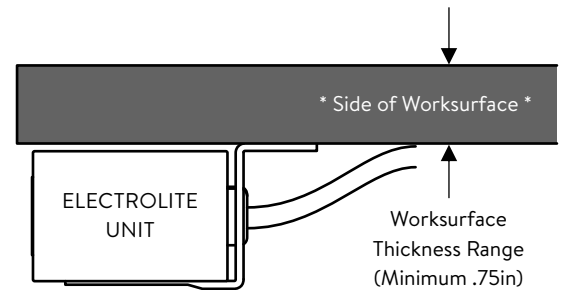
ELEVATION DETAIL
